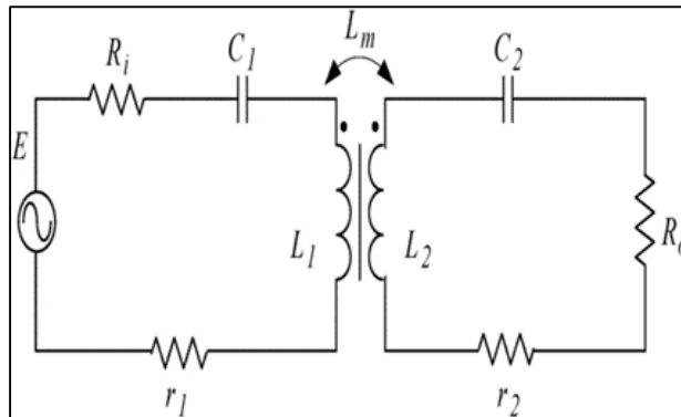
Fig. 4: Equivalent circuit of the resonant magnetic coupling system
