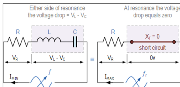
Fig. 3a: LC series connection without
