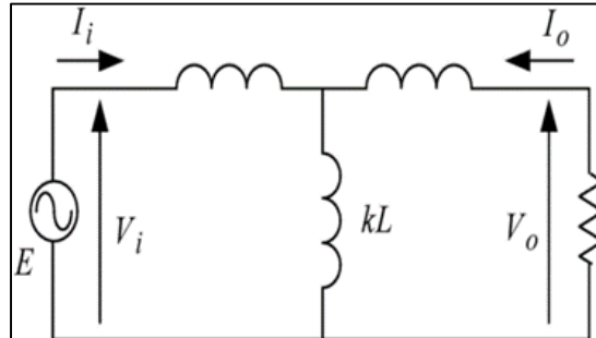
Fig. 1: Equivalent circuit diagram of an electromagnetic induction method
