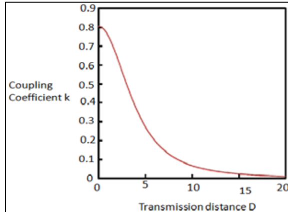
Fig. 8: Relationship between the coupling coefficient and the transmission distance
