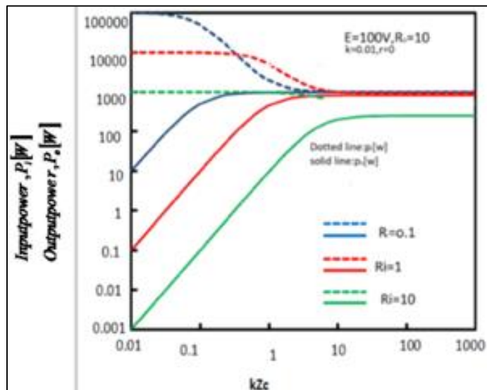
Fig. 5: Output power characteristics
