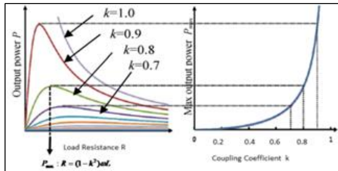
Fig. 2: Output power characteristics
