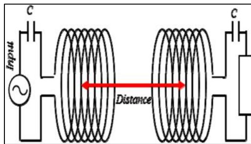
Fig. 6: schematic diagram of the experimental setup
