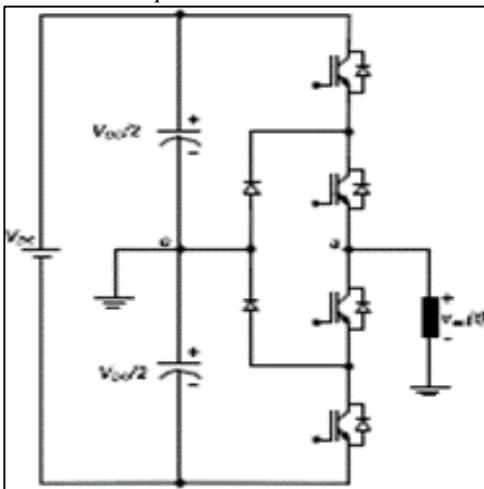
Fig. 5: Single-phase nine-level diode clamped inverter
