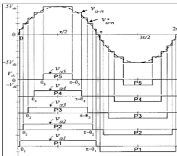
Fig. 4: Output Waveform of Cascaded H-Bridge Multilevel inverter
