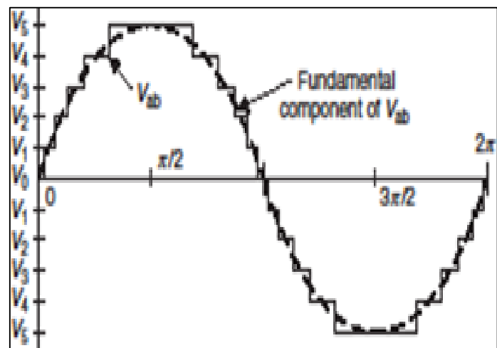
Fig. 6: Output waveform for three-phase six-level diode clamped inverter
