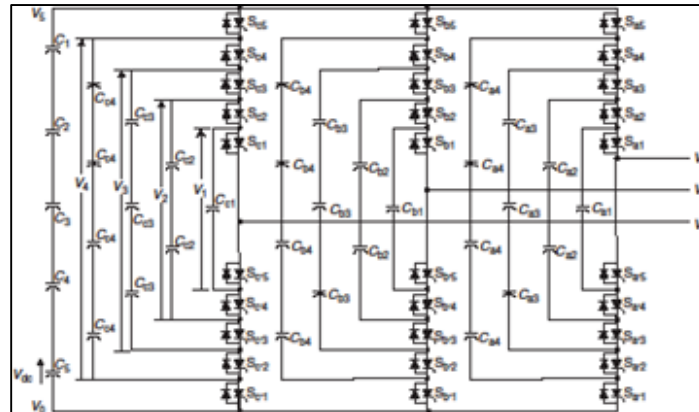
Fig. 7: Three-phase six-level flying capacitor inverter
