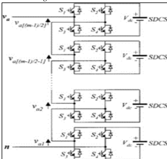
Fig. 3: Single Phase m -level Cascaded H- Bridge Multilevel inverter
