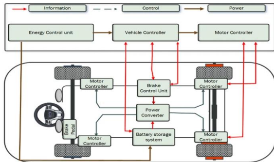
Fig 1: Basic Configuration for Driving Control Logic
