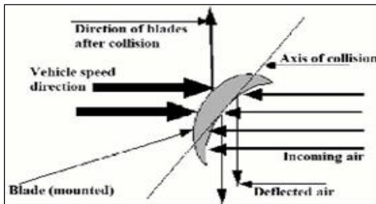
Fig. 3: working model of blades of wind turbine
