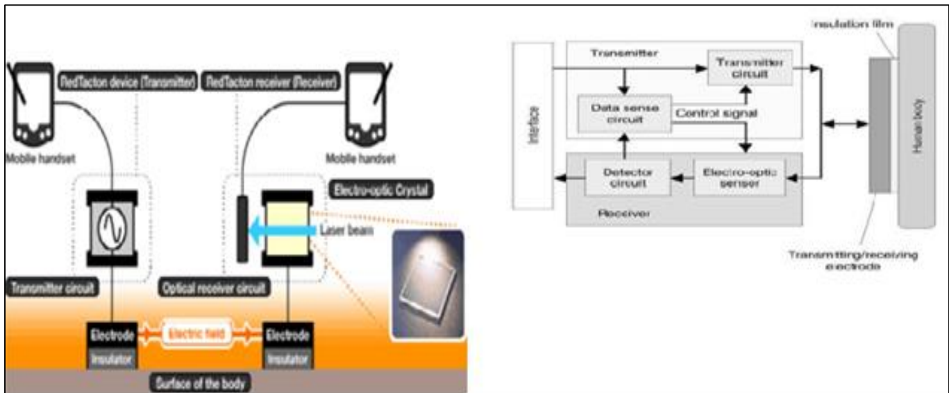
Fig. 2: Electro-Optic field sensor combined with Electro-Optic crystal and laser light
